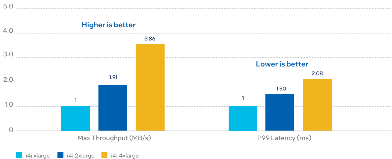
Figure 4: Intel® AWS i4i Instances scaling (LZ4 compression).
